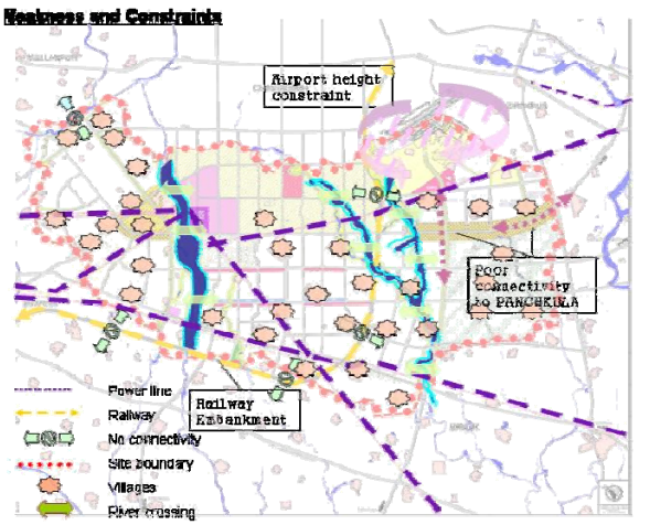
Figure 2.5: Presence of High Tension Power Lines Across Site
