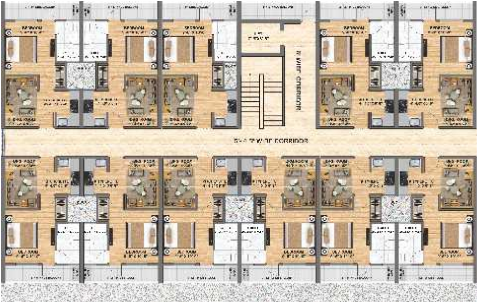
Typical Cluster Floor Plan - 1st & 2nd Floor
