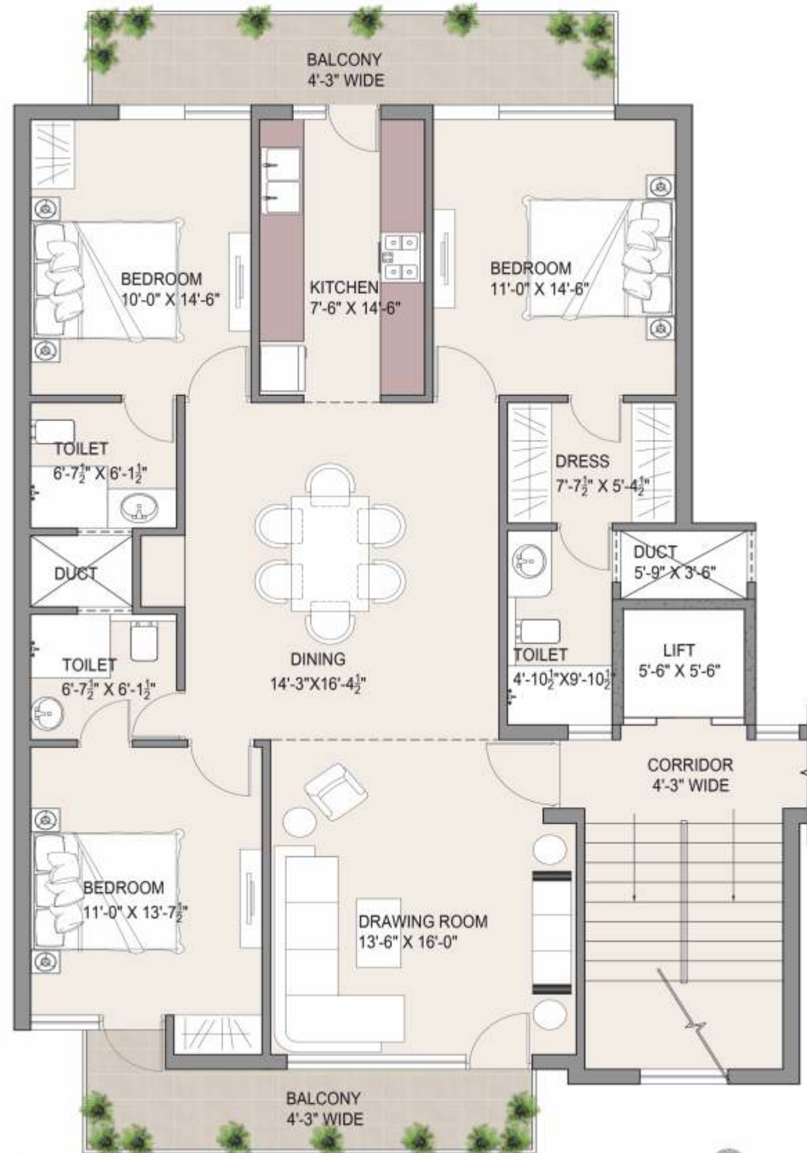
TYPICAL FLOOR PLAN 3BHK
