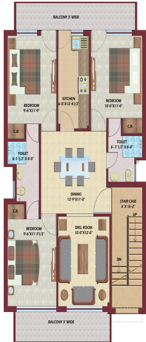
FIRST & SECOND FLOOR PLAN SUPER AREA: 1225 Sq. Ft. (approx)
