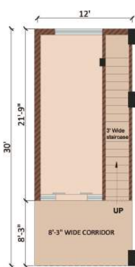
Ground Floor Plan Covered Area: 360 sq.ft. Floor to Floor Height: 11 ft.
